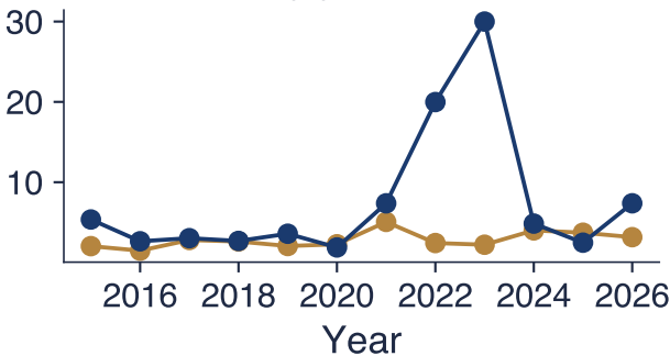
Student-t \hat{v} by year (capped at 30)
