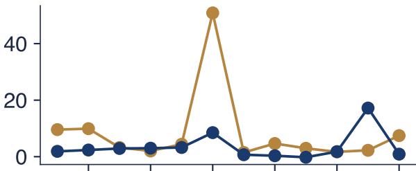
Excess kurtosis by year
