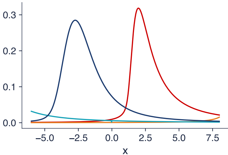
S1: \beta = 0.8 , \gamma = 1 , \delta = 0
