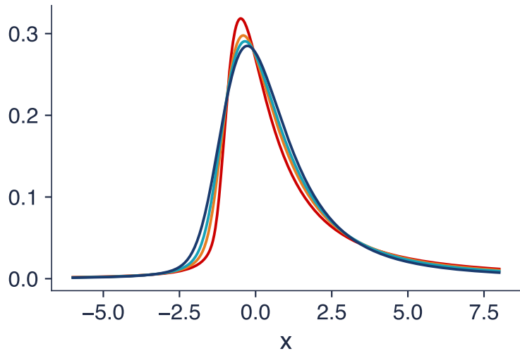
S0: \beta = 0.8 , \gamma = 1 , \delta = 0
