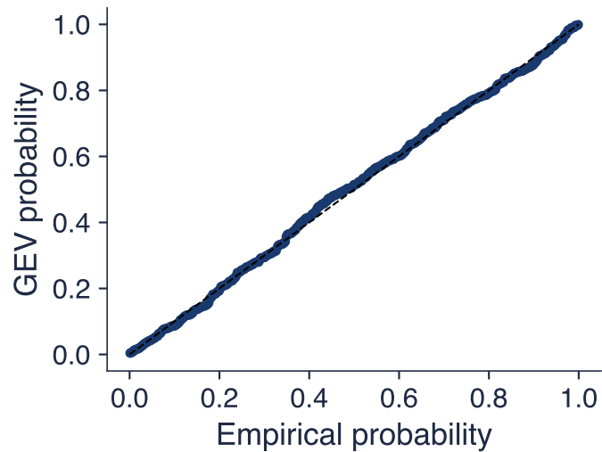
PP plot
