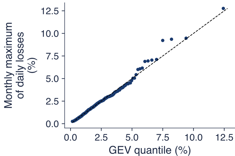
QQ plot
