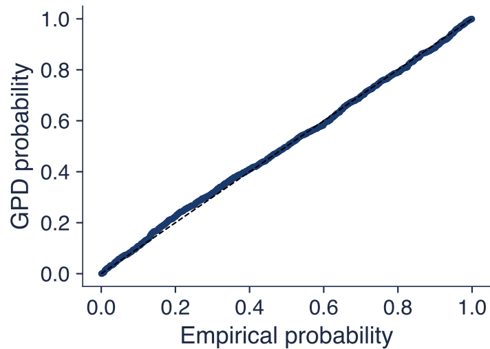
PP plot
