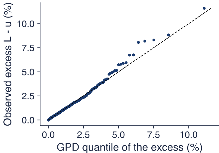
QQ plot
