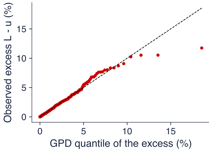
QQ plot of the excesses
