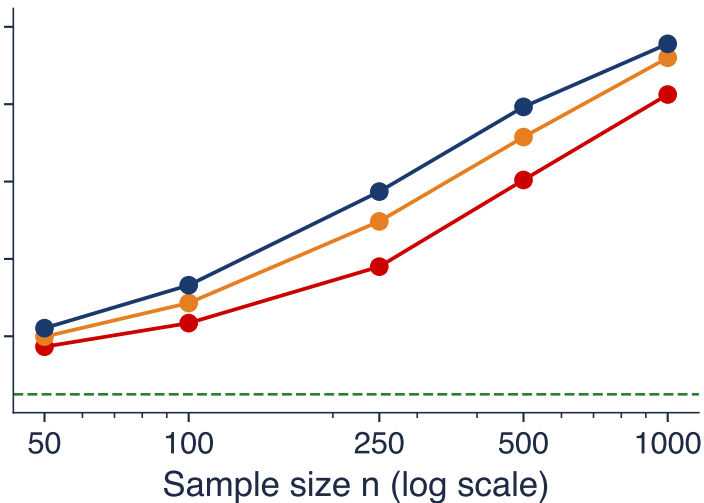
Normal data, 2% of days with 4x volatility
