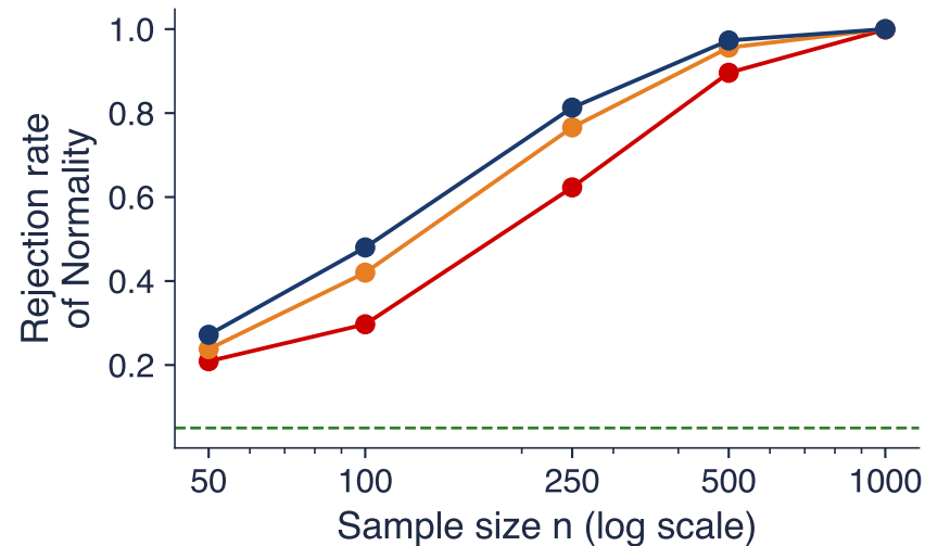
Student-t data, \nu = 5
