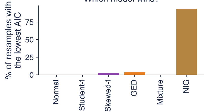
Which model wins?
