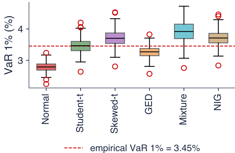
Bootstrap spread of VaR 1%
