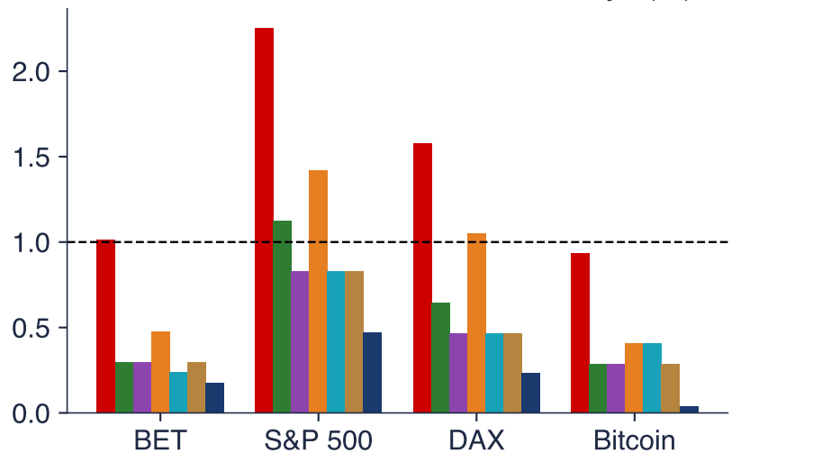
VaR 1% exceedances on the test days (%)
