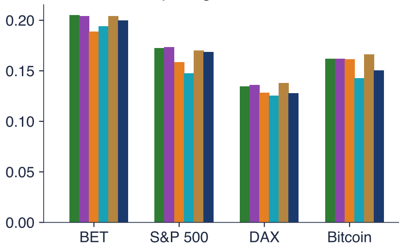
Out-of-sample log score minus Normal
