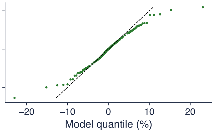
S&P 500: QQ plot, Student-t
