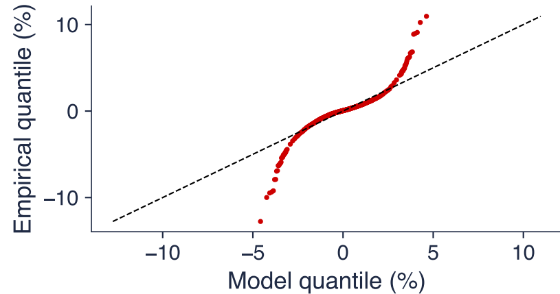
S&P 500: QQ plot, Normal
