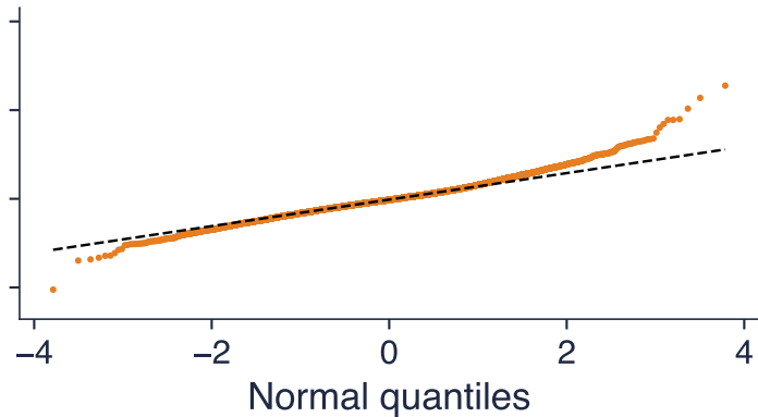
EMA, \lambda = 0.96
