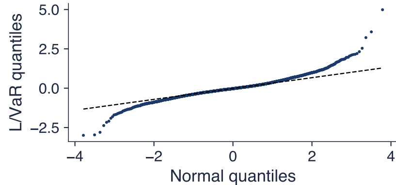
RMA, h = 250
