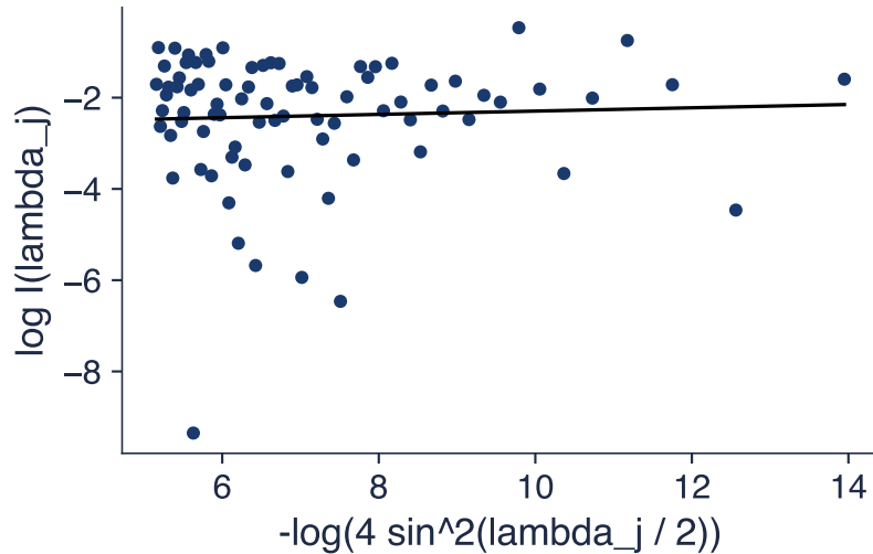
returns r: slope d = 0.04 (SE 0.07)
