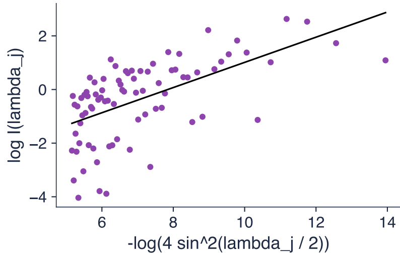
absolute returns lrl: slope d = 0.47 (SE 0.07)
