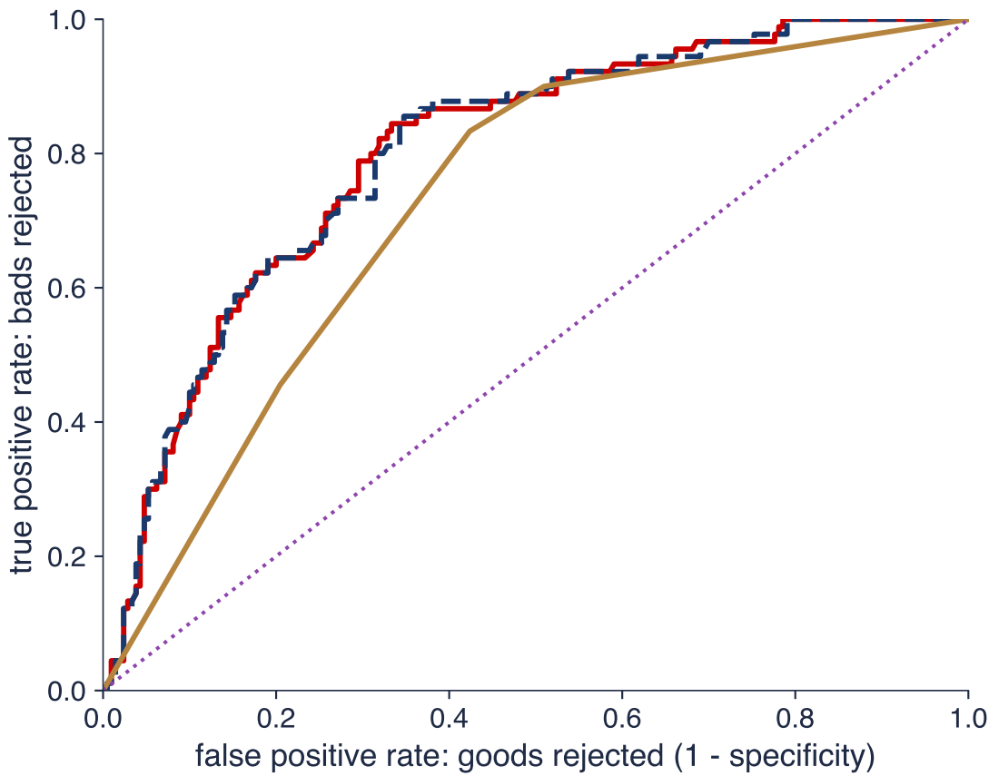
— WoE logit (AUC = 0.801) — checking account only (AUC = 0.728) - - Fisher LDA (AUC = 0.801) ..... random score (AUC = 0.5)
