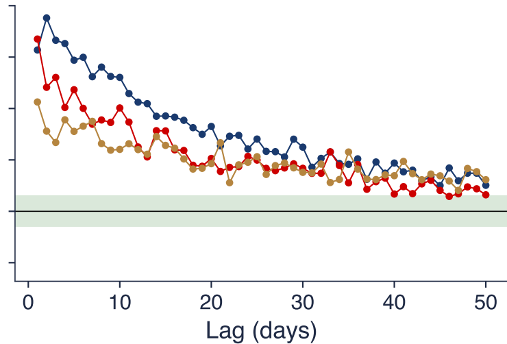
Absolute returns |r_t|
