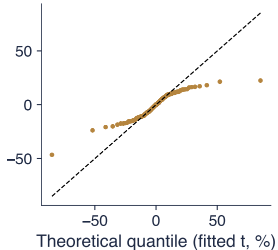
Bitcoin vs t(2.2)
