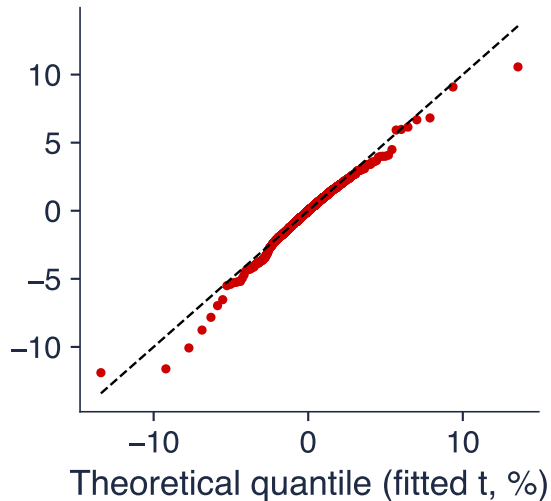
BET vs t(3.0)
