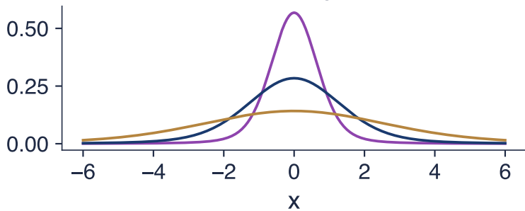
alpha = 1.7, beta = 0: the effect of gamma
