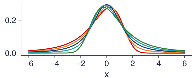
alpha = 1.3, gamma = 1: the effect of beta
