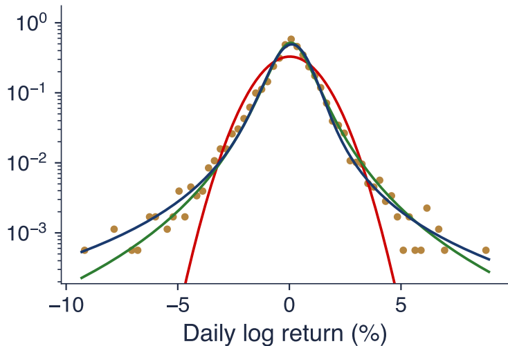
S&P 500: \hat{\alpha} = 1.54
