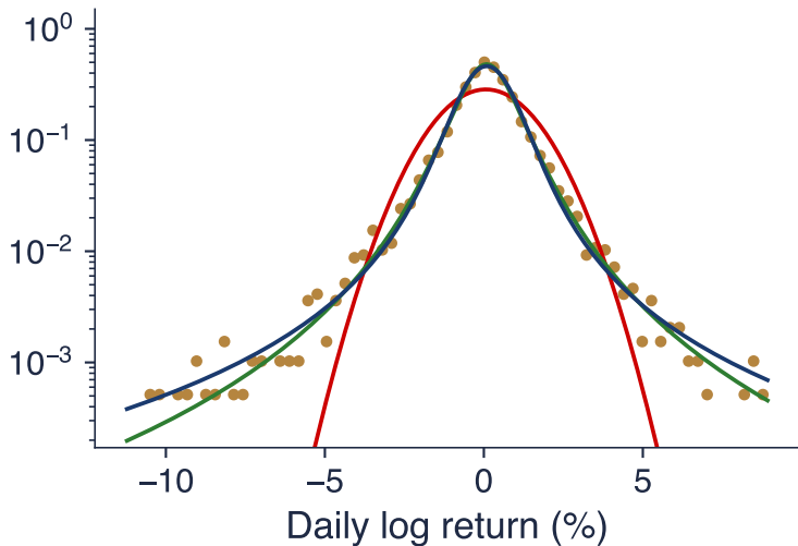
BET: \hat{\alpha} = 1.49
