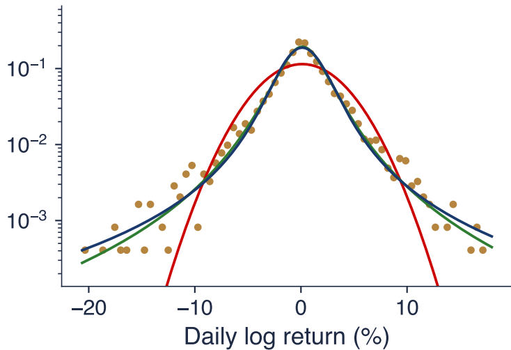
Bitcoin: \hat{\alpha} = 1.41
