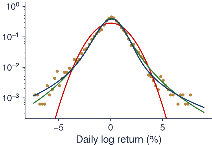
DAX: \hat{\alpha} = 1.61
