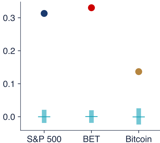
\text{Corr}(r_t^2, r_{t-1}^2)
