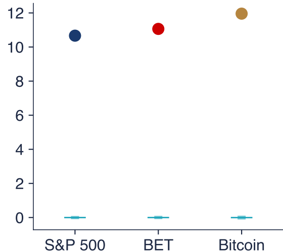
excess kurtosis
