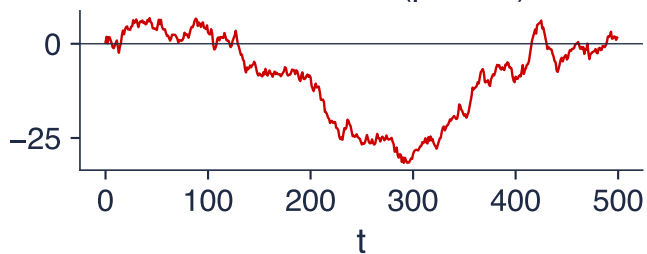
random walk ( \phi = 1 )
