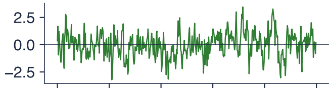
AR(1), \phi = 0.5
