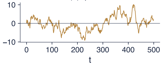
AR(1), \phi = 0.95
