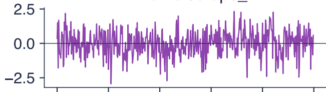
white noise \epsilon_{s_t}
