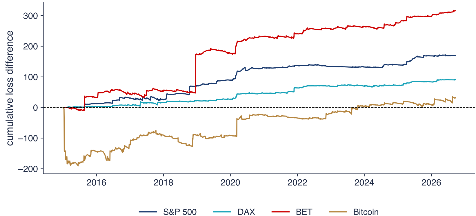
Cumulative QLIKE(EWMA) - QLIKE(GARCH-t): rising = GARCH-t better
