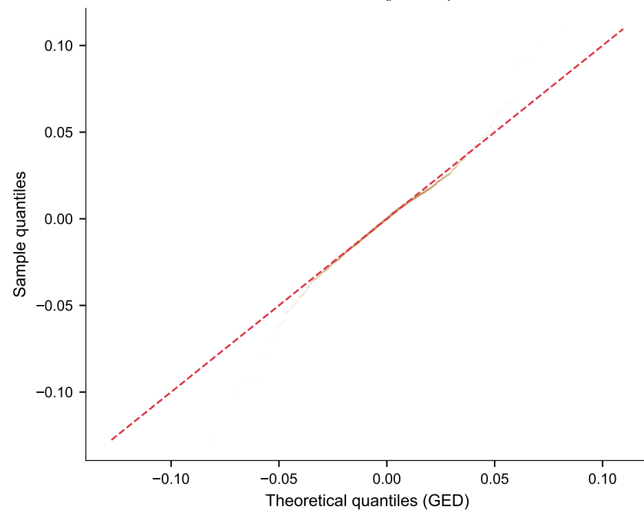
C. GED QQ ( \beta=0.87 )
