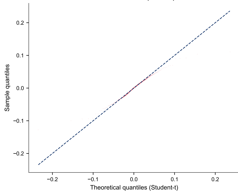
B. Student-t QQ (df=2.64)
