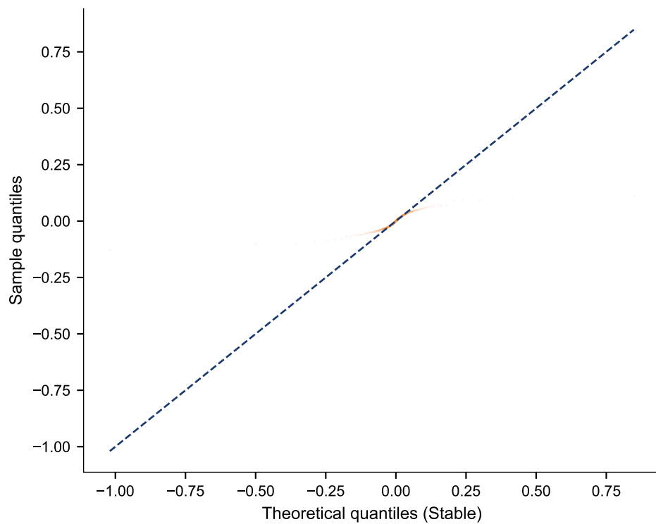
D. Stable QQ ( \alpha=1.54 )
