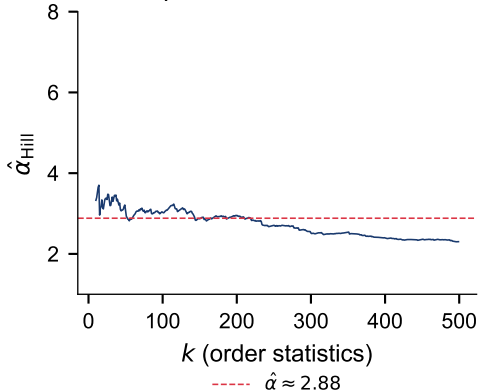
Hill plot — S&P 500 losses
