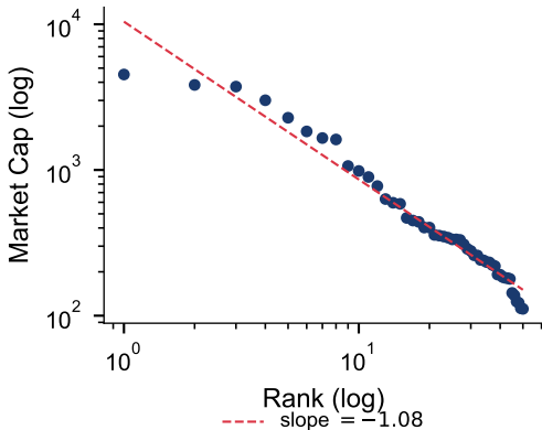
Zipf's law — log-log
