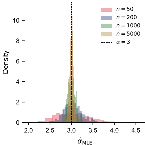
MLE convergence
