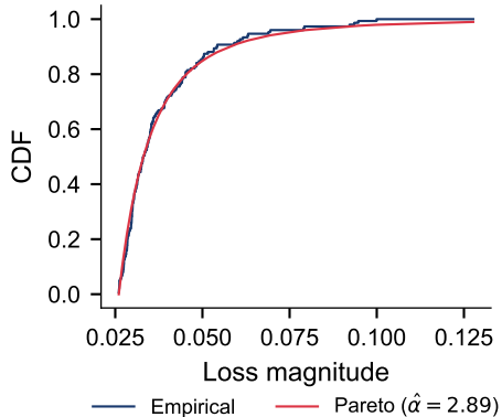
Tail CDF fit (top 5%)
