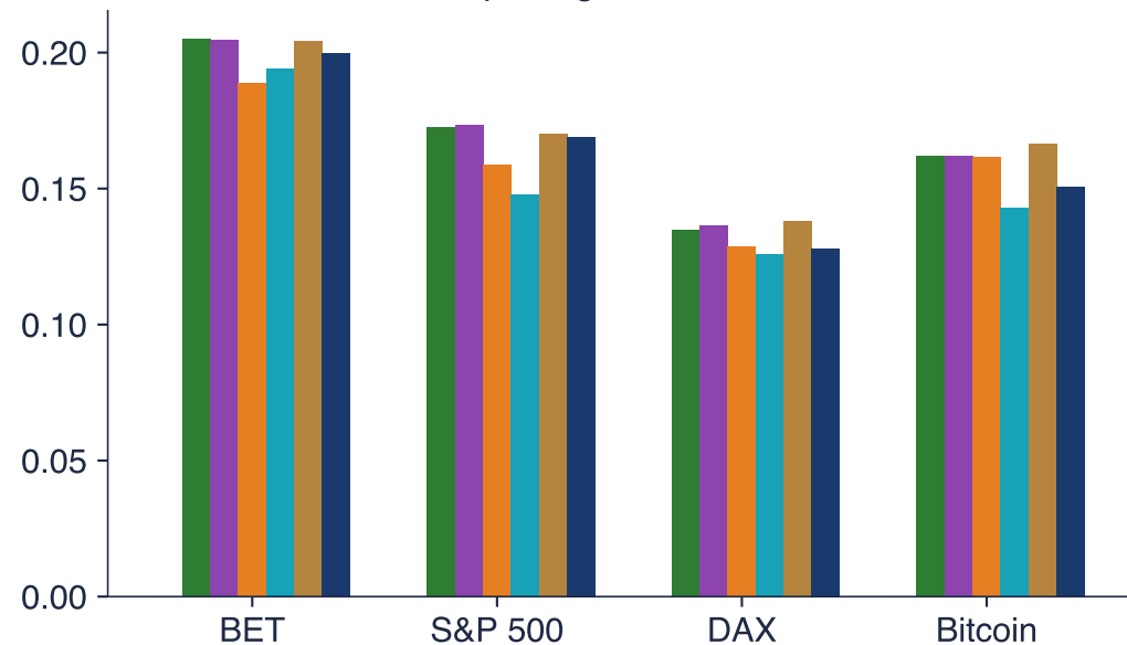
Out-of-sample log score minus Normal
