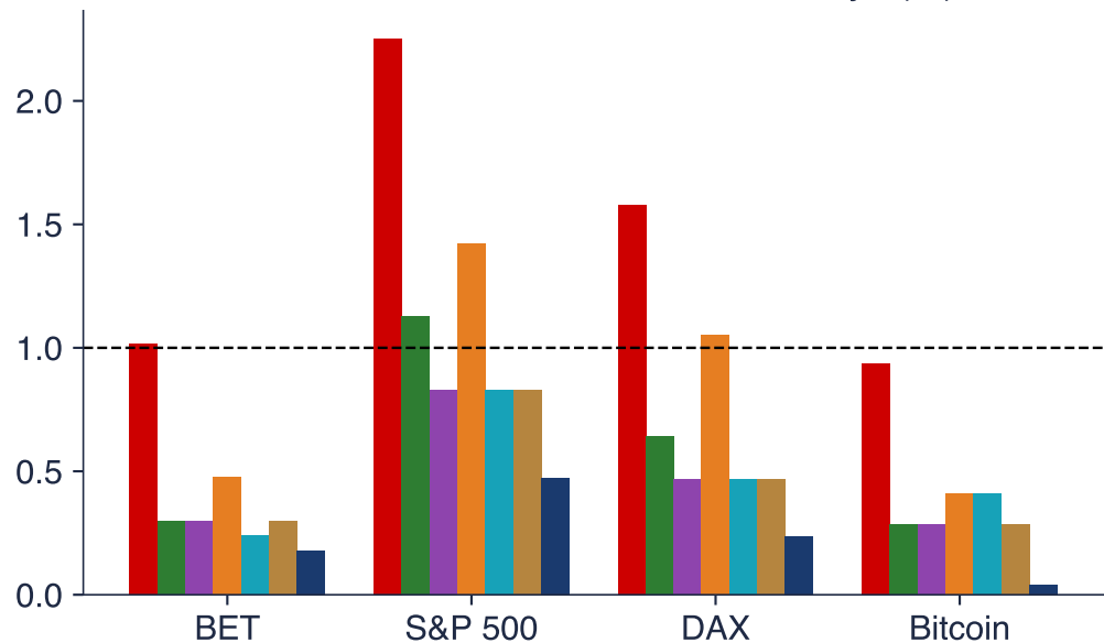
VaR 1% exceedances on the test days (%)
