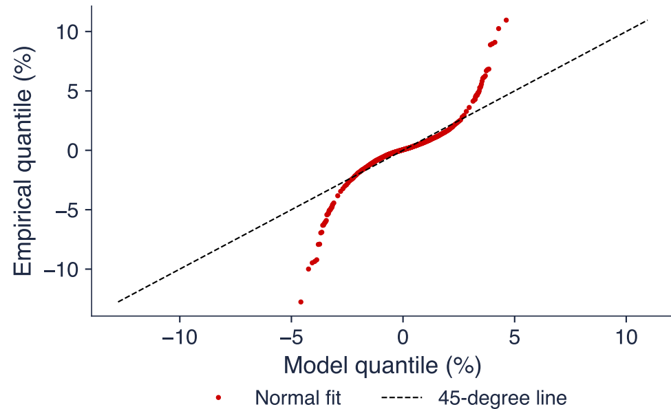
S&P 500: QQ plot, Normal
