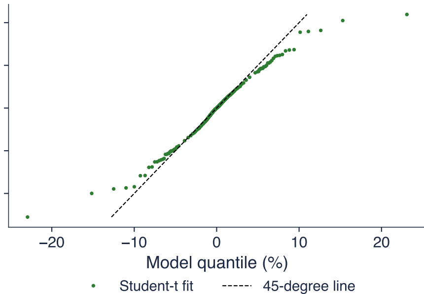
S&P 500: QQ plot, Student-t
