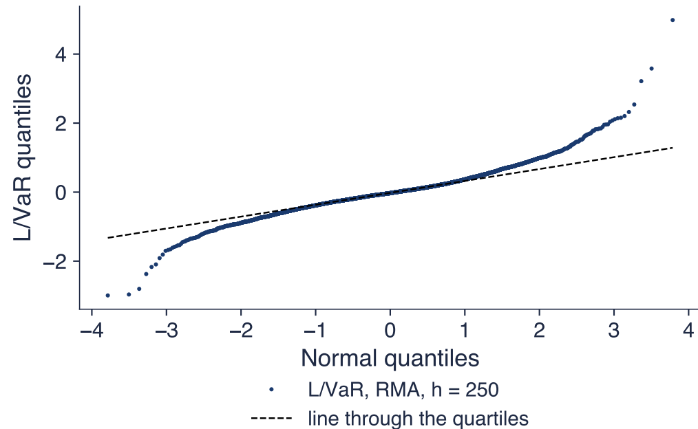
RMA, h = 250
