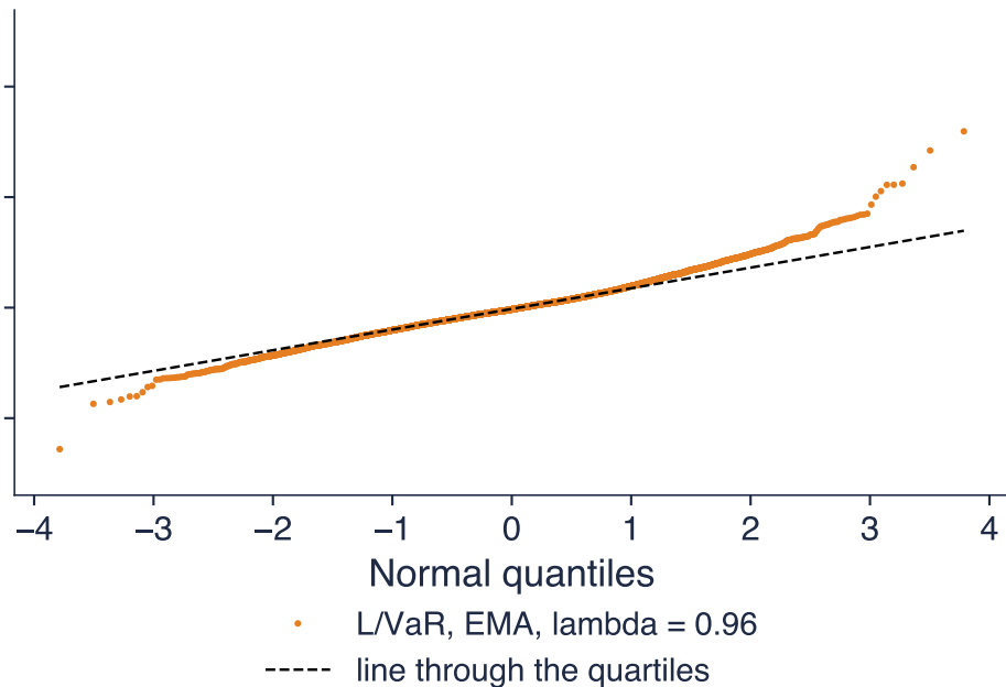
EMA, \lambda = 0.96
