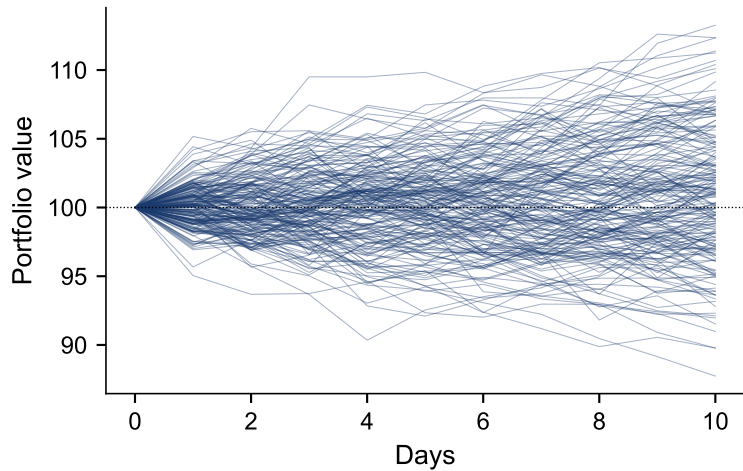
200 Monte Carlo paths (10-day horizon)
