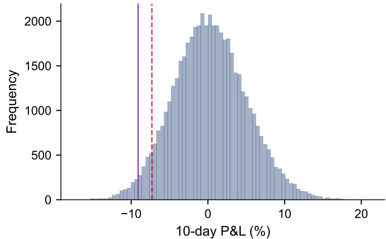
P&L histogram with MC VaR and ES (5%)
