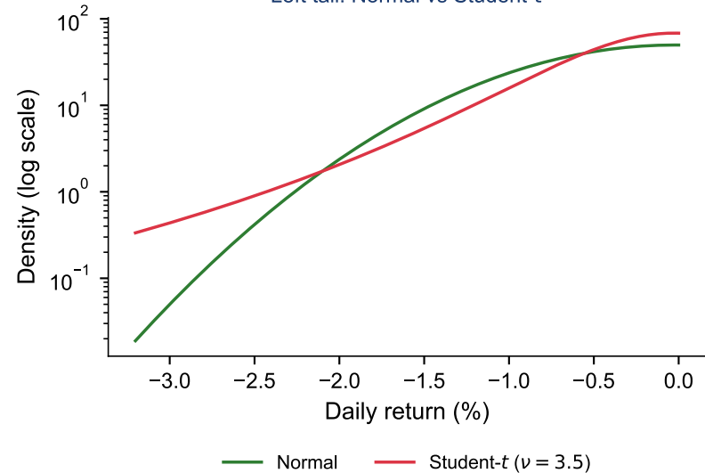
Left tail: Normal vs Student-t
