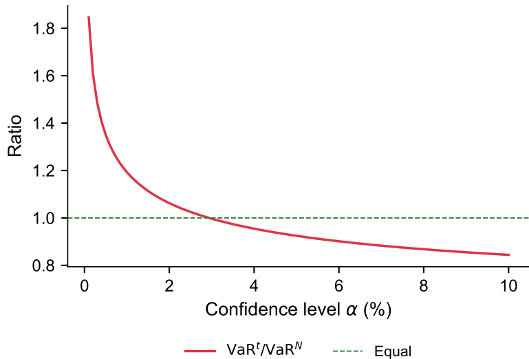
Student-t VaR vs Normal VaR ( \nu = 3.5 )
