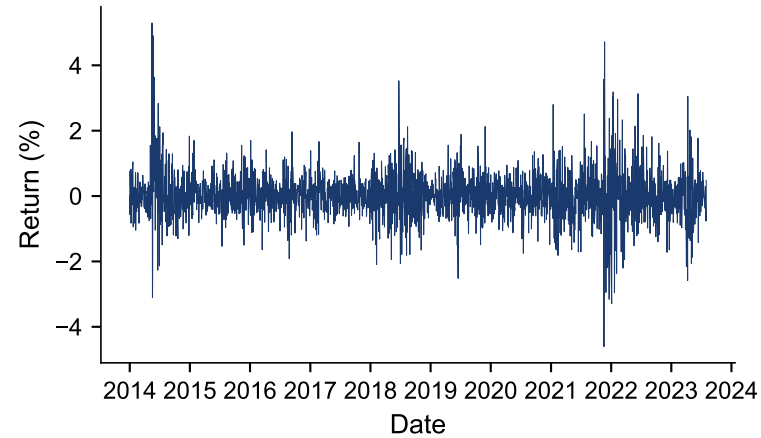
Simulated GARCH- t returns
