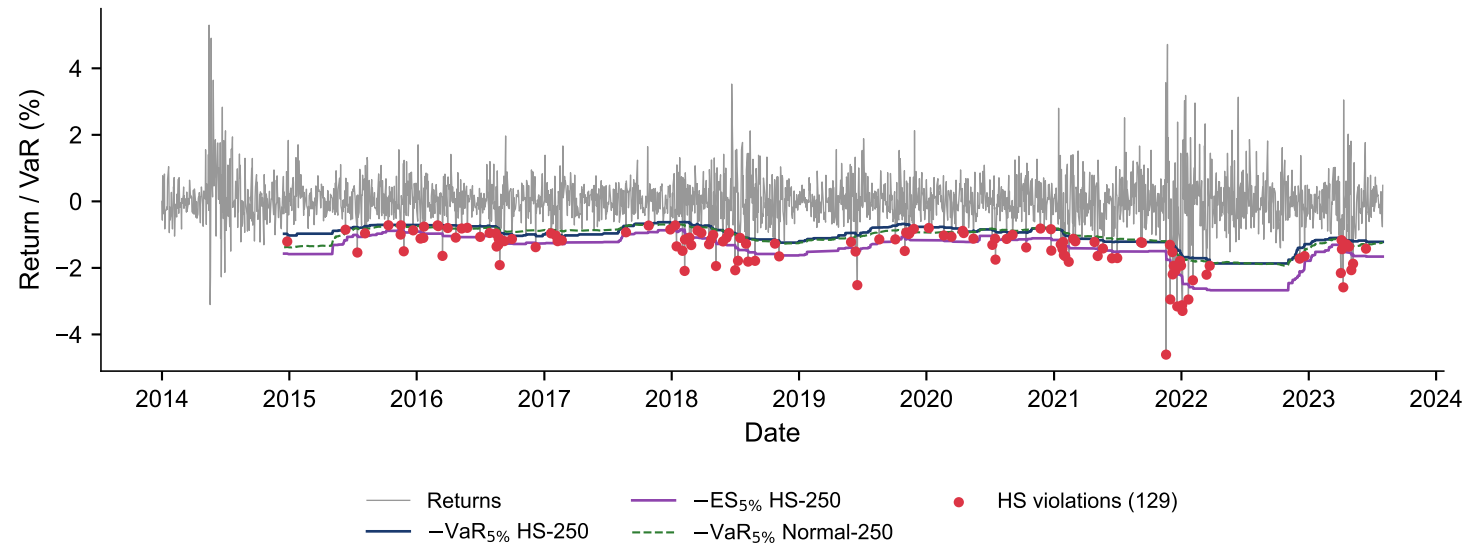
Rolling 250-day VaR and ES at 5% with realised violations
