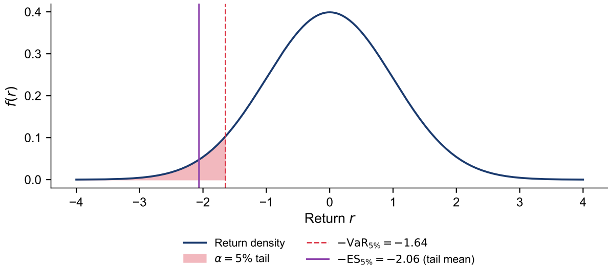
VaR vs Expected Shortfall
