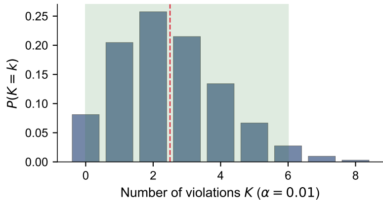
Binomial(250, 0.01)
