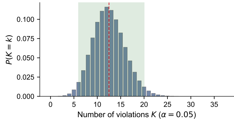
Binomial(250, 0.05)
