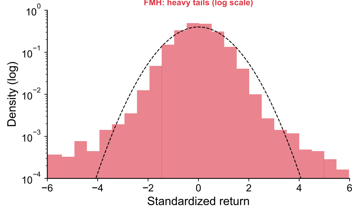
FMH: heavy tails (log scale)
