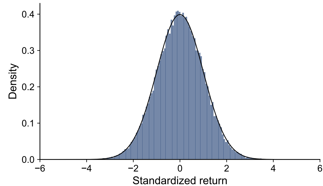
EMH: Gaussian distribution
