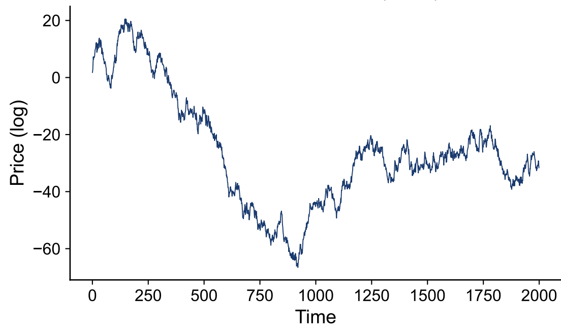
EMH: Gaussian random walk ( H = 0.5 )
