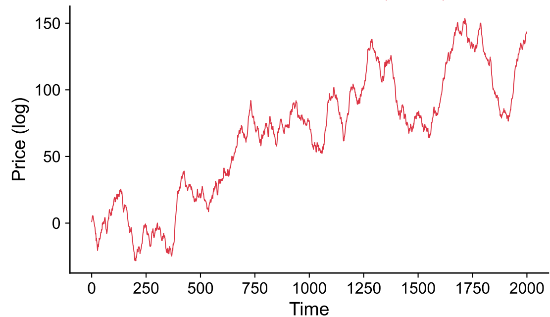
FMH: fractional Brownian motion ( H = 0.75 )
