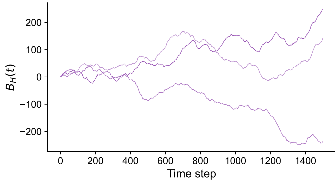
H = 0.9 (strongly persistent)
