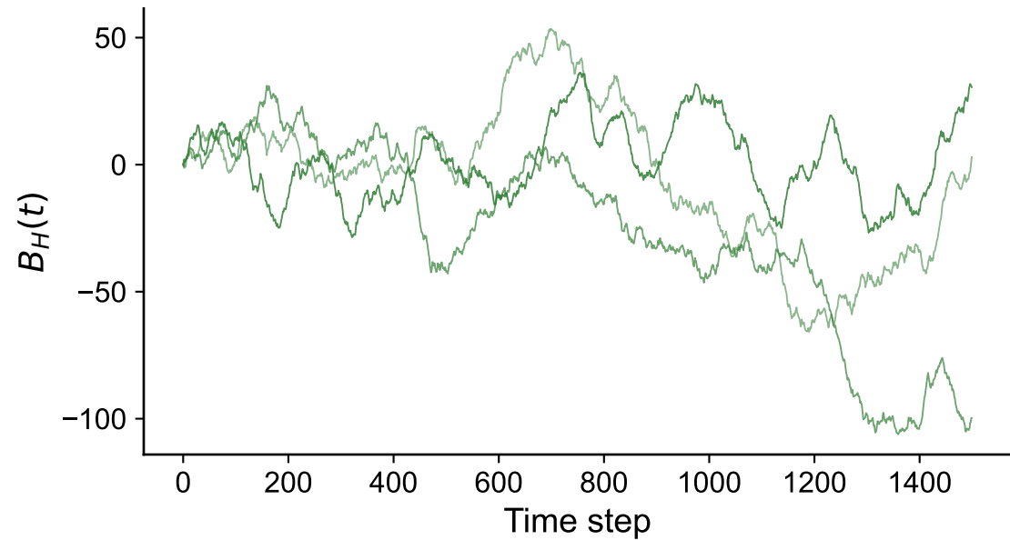
H = 0.7 (weakly persistent)
