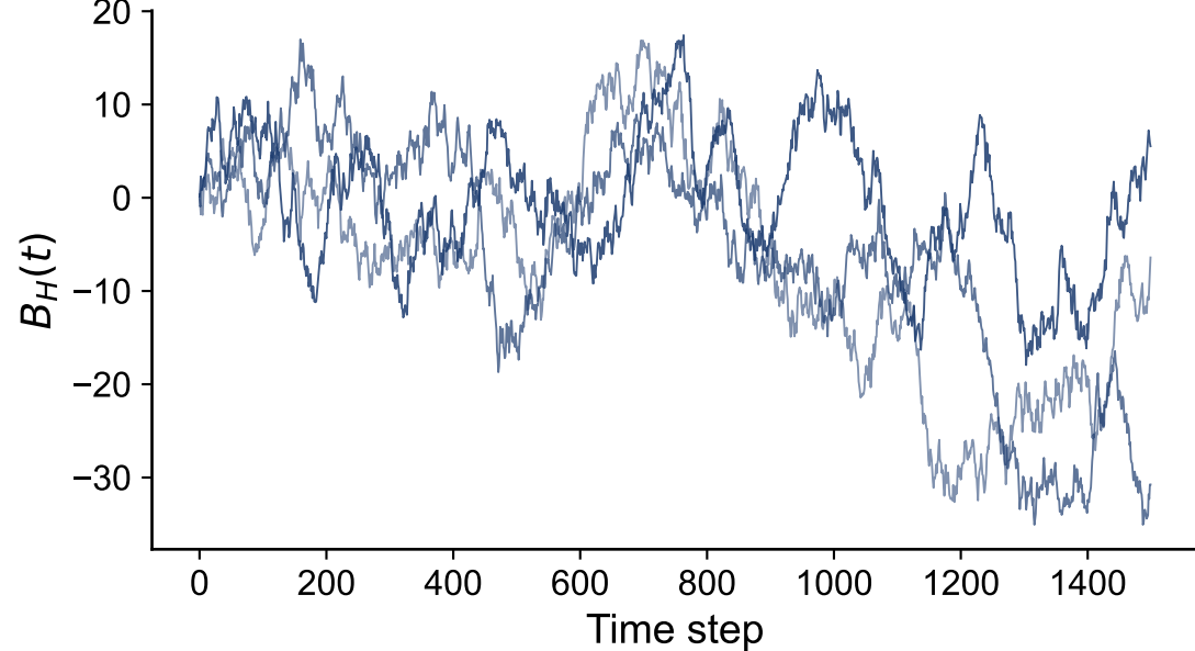
H = 0.5 (random walk (Brownian))
