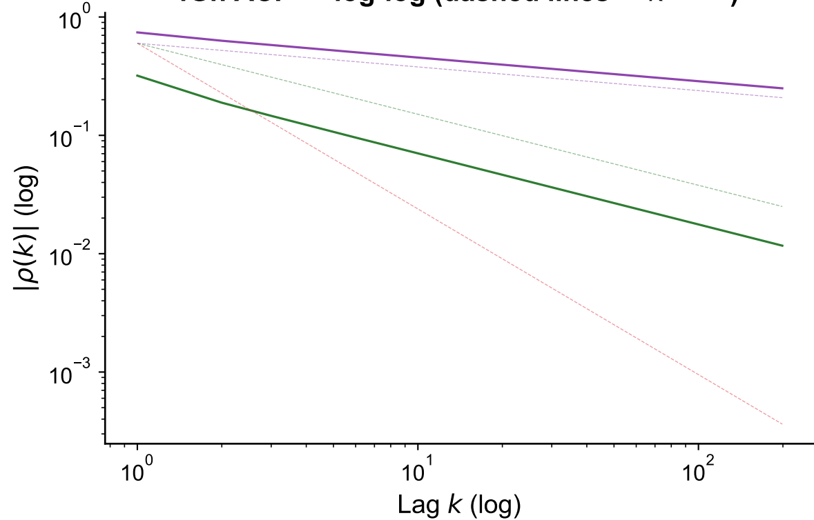
fGn ACF — log-log (dashed lines \propto k^{2H-2} )
