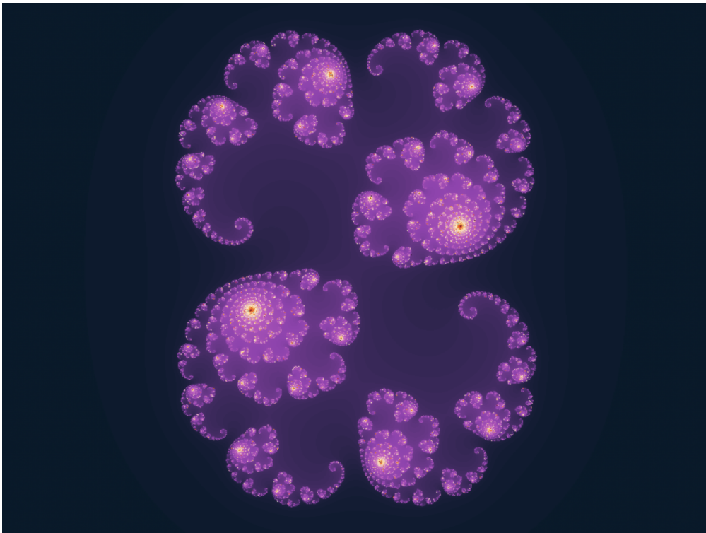
C: c = 0.285 + 0.01i (Connected)
