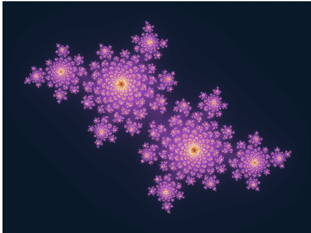
D: c = -0.4 + 0.6i (Spiral structure)
