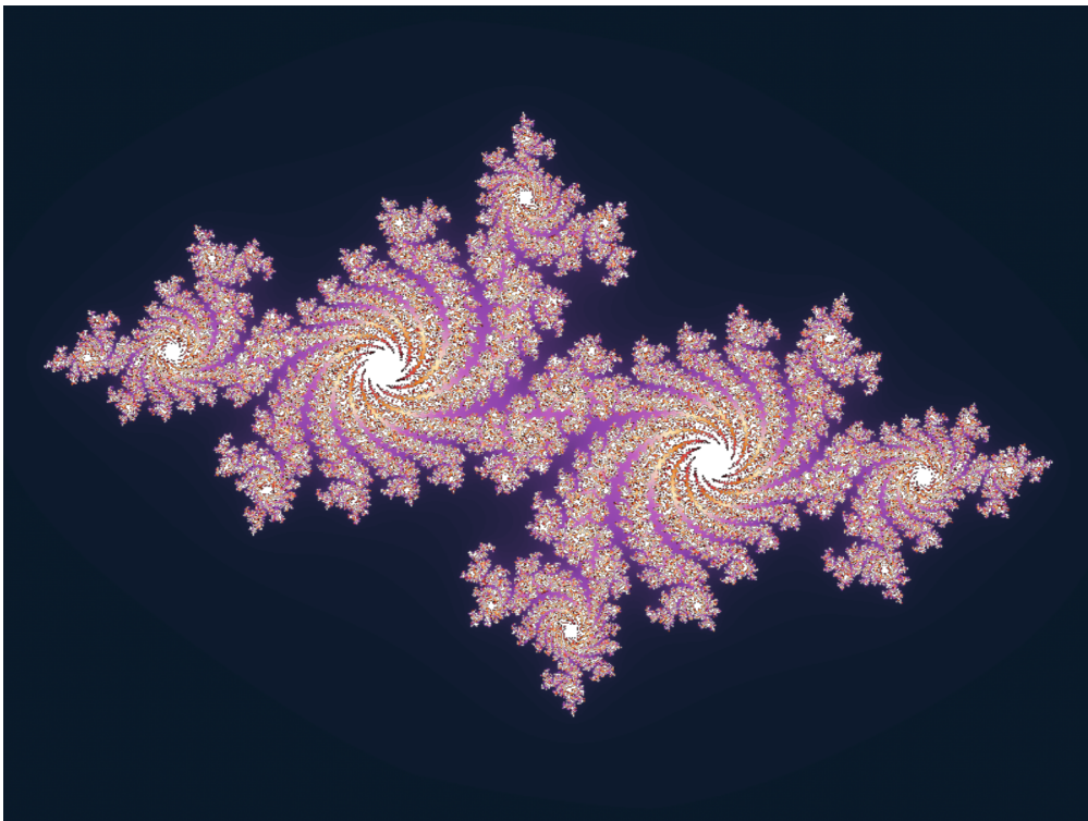
A: c = -0.7 + 0.27015i (Dendrite-like)
