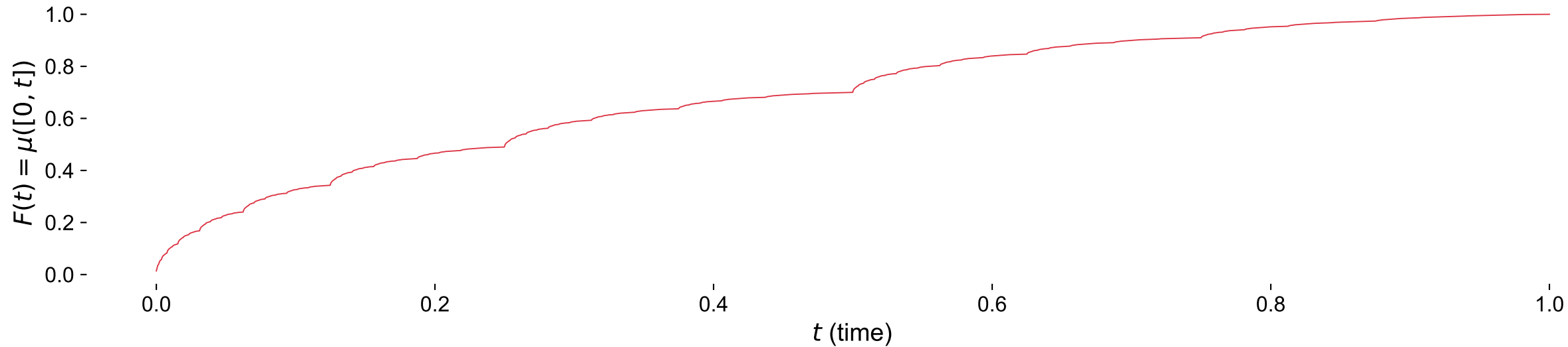
Cumulative function (devil's staircase)
