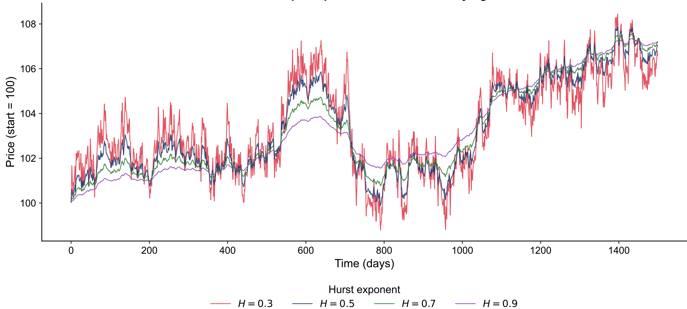
Simulated price paths under fBm for varying H
