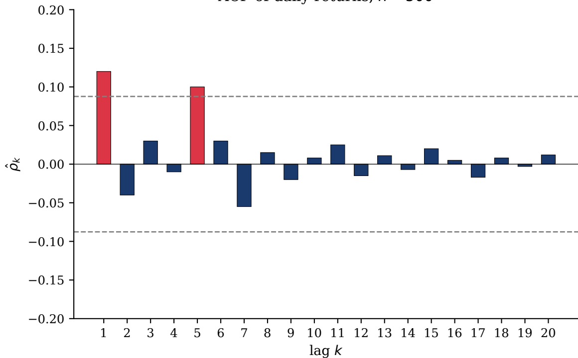
ACF of daily returns, n = 500
