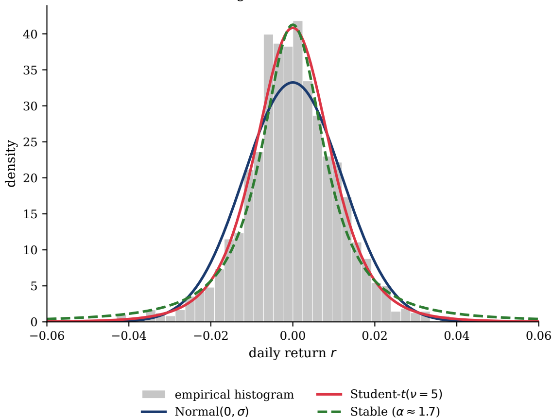
Returns histogram vs theoretical densities
