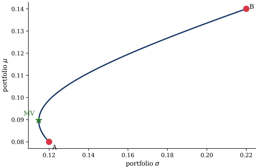
Efficient frontier --- 2 assets, \rho = 0.25
