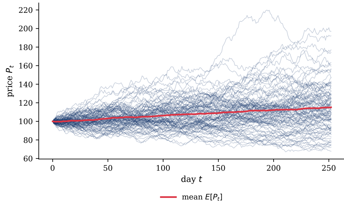
Monte Carlo --- 100 GBM paths (1 year)
