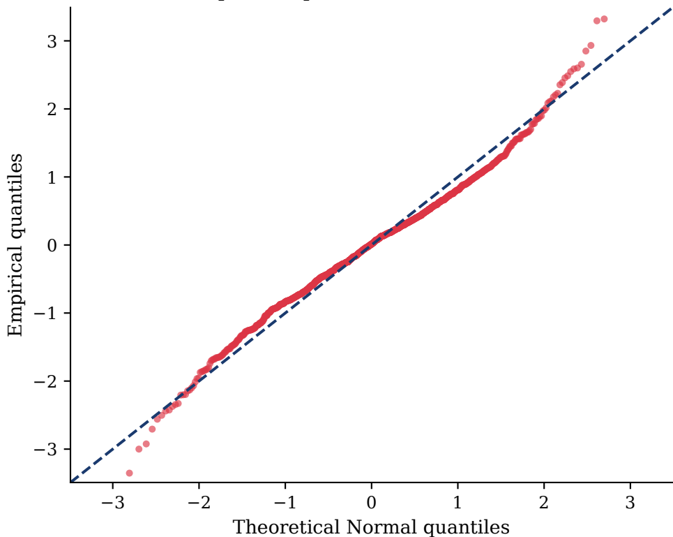
QQ-plot: empirical returns vs Normal
