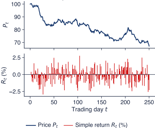
Simulated daily closes
