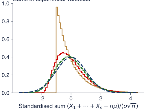
Sums of exponential variables
