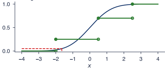
CDF: grows from 0 to 1
