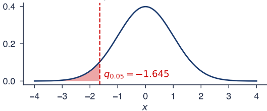
Continuous: density f of N(0, 1)
