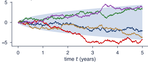
Wiener process W(t) \sim N(0, t)
