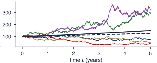
GBM, \mu = 8\% , \sigma = 25\% , S_0 = 100
