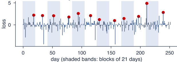
Block maxima: the largest loss of each month
