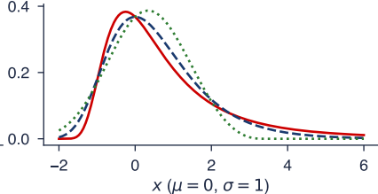
GEV densities
